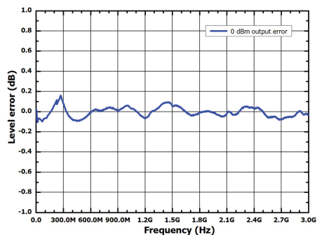
Measured at 0 dBm,level error vs.frequency
