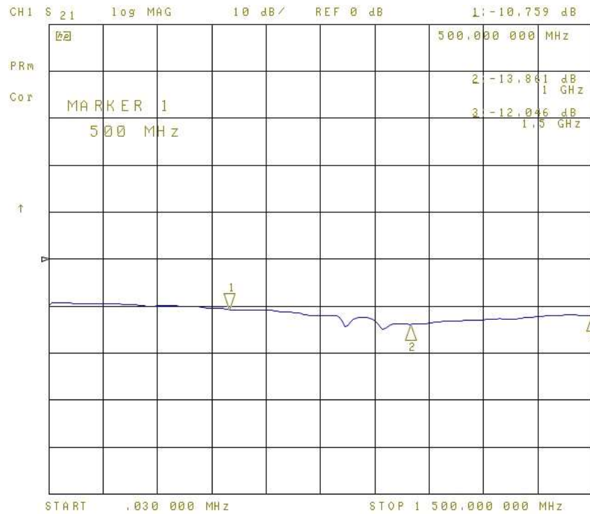
Picture 7 – TBFL1, attenuation, IS211, 30 kHz – 1.5 GHz
