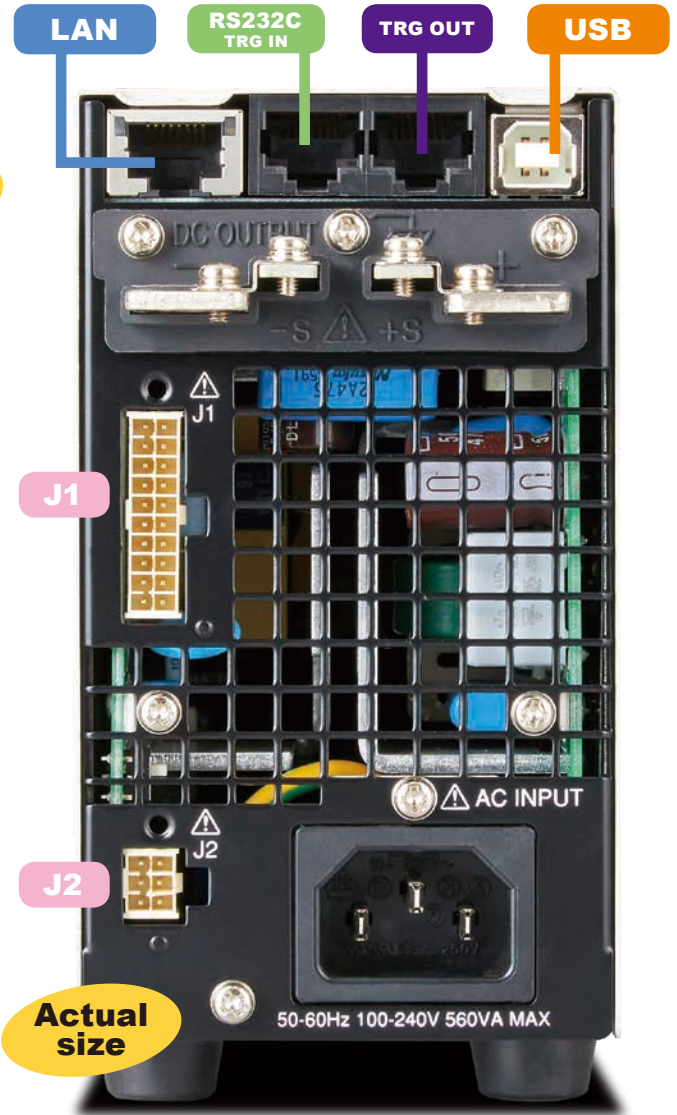
Rear Panel : 400 W model
