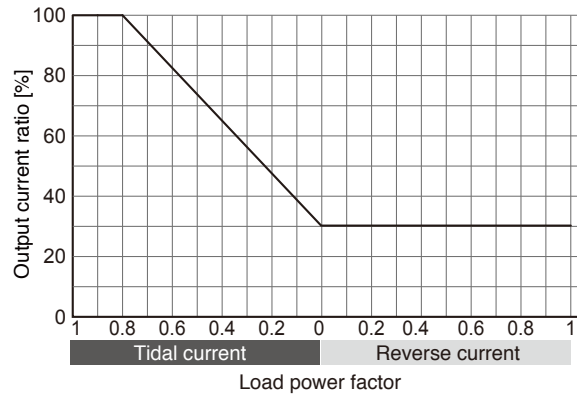
■ Load power factor versus rated output current characteristics
